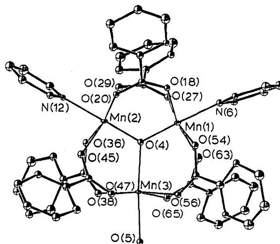
Figure 1. The structure of \text{Mn}_3\text{O}(\text{O}_2\text{CPh})_6(\text{py})_2(\text{H}_2\text{O}) . \text{Mn}(3) is the \text{Mn}^{\text{II}} center, and \text{O}(5) is the \text{H}_2\text{O} molecule. \text{Mn}(1)\cdots\text{Mn}(2) , 3.218 (4) Å; \text{Mn}(1)\cdots\text{Mn}(3) , 3.418 (5) Å; \text{Mn}(2)\cdots\text{Mn}(3) , 3.396 (5) Å.
