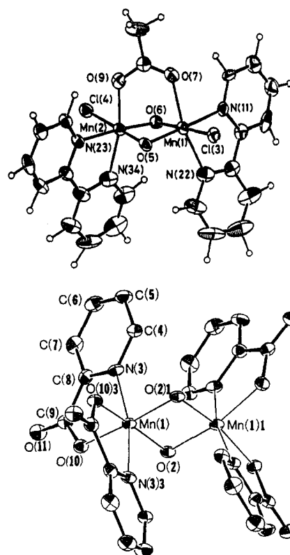
Figure 5. The structures of complex 6 (top) and complex 7 (bottom). For 6: \text{Mn}(1)\cdots\text{Mn}(2) , 2.567 (2) Å. For 7: \text{Mn}(1)\cdots\text{Mn}(11) , 2.747 (2) Å. (Reprinted with permission from ref 20a. Copyright 1988 Royal Society of Chemistry.)
